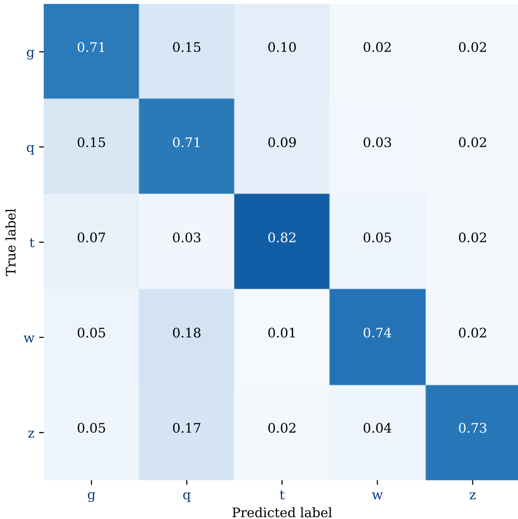
Confusion Matrix of Jet-tagger: HGQ with 1001 EBOPs
